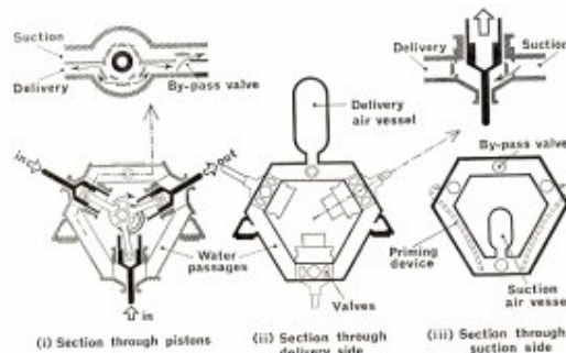
Fig. 1-8. Diagrams showing the construction of a reciprocating fire pump.
