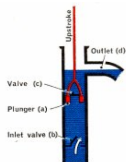
Fig. 1-5. Diagram showing the operation of a lift pump.
