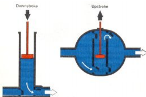
Fig. 1-3. Diagram showing the operation of a force pump. Left: single acting. Right: double acting.
