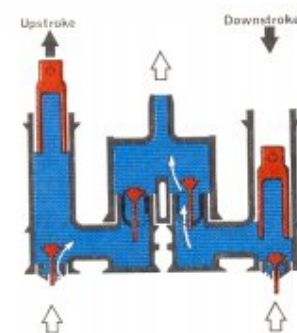
Fig. 1-1. Early double-cylinder force pump.
